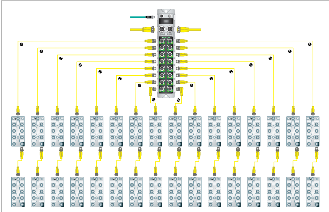
Figure 5: Balluff expanded I/O with 480 points
