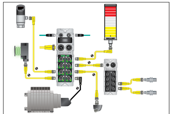
Figure 11: IO-Link distributed modular architecture
